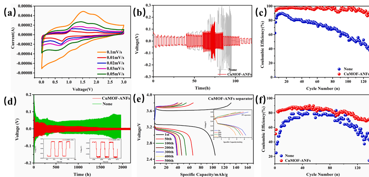
Fig. 4. (a) Cyclic voltammety (CV) scans of the Li-Cu half-cell (b) Rate performance of Li-Li battery (c) Coulombic efficiency of Li plating test with CuMOF-ANFs separator cells (red) and normal cells (blue) at current densities of 1 \text{ mA/cm}^2 ( 1 \text{ mAh/cm}^2 ) (d) Cycling performance of the Li|Li cells with different separators at a current density of 1 \text{ mA/cm}^2 (e) Voltage profiles of CuMOF-ANFs separator and PP separator (f) Coulombic efficiency of Li plating test with CuMOF-ANFs separator cells (red) and normal cells (blue) at current densities of 1 \text{ mA/cm}^2 ( 1 \text{ mAh/cm}^2 ).
