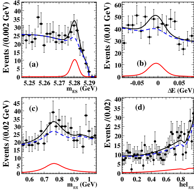
FIG. 1 (color online). Projections of the multidimensional fit onto (a) m_{ES} , (b) \Delta E , (c) dipion invariant mass ( m_1 is shown, distribution of m_2 is similar), and (d) cosine of the helicity angle ( \cos\theta_1 is shown), after a requirement on the signal-to-background probability ratio with the plotted variable excluded. This requirement enhances the fraction of signal events in the sample. The data points are overlaid by the solid black line, which corresponds to the full PDF projection. The individual B^0 \rightarrow \rho^0 \rho^0 PDF component is also shown with a solid red line. The sum of all other PDFs (including B^0 \rightarrow \rho^0 f_0 and B^0 \rightarrow f_0 f_0 components) is shown as the dashed blue line. The D -meson veto causes the acceptance dip seen in (d).
